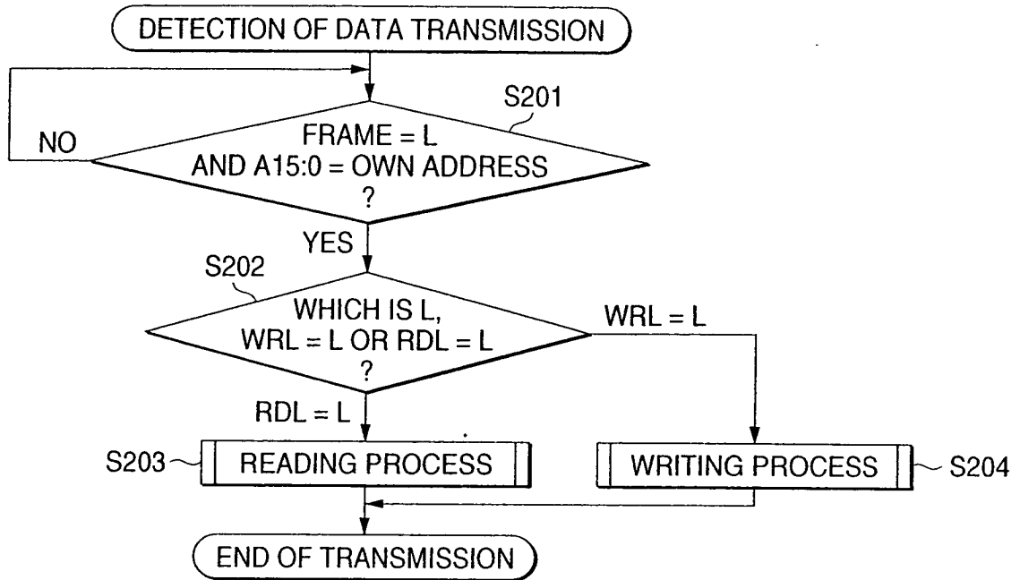
FIG. 18 PRIOR ART
